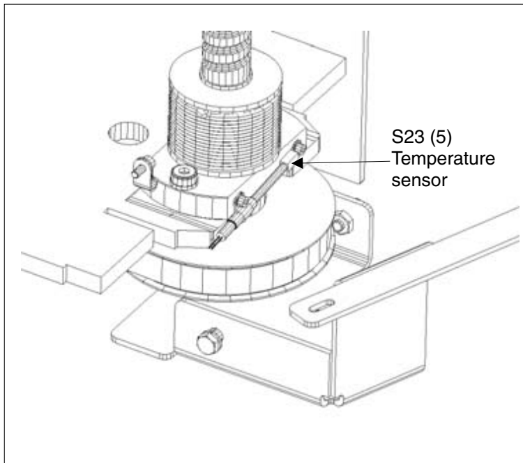
Fig. 27: Switch location, lower spindle part S23
