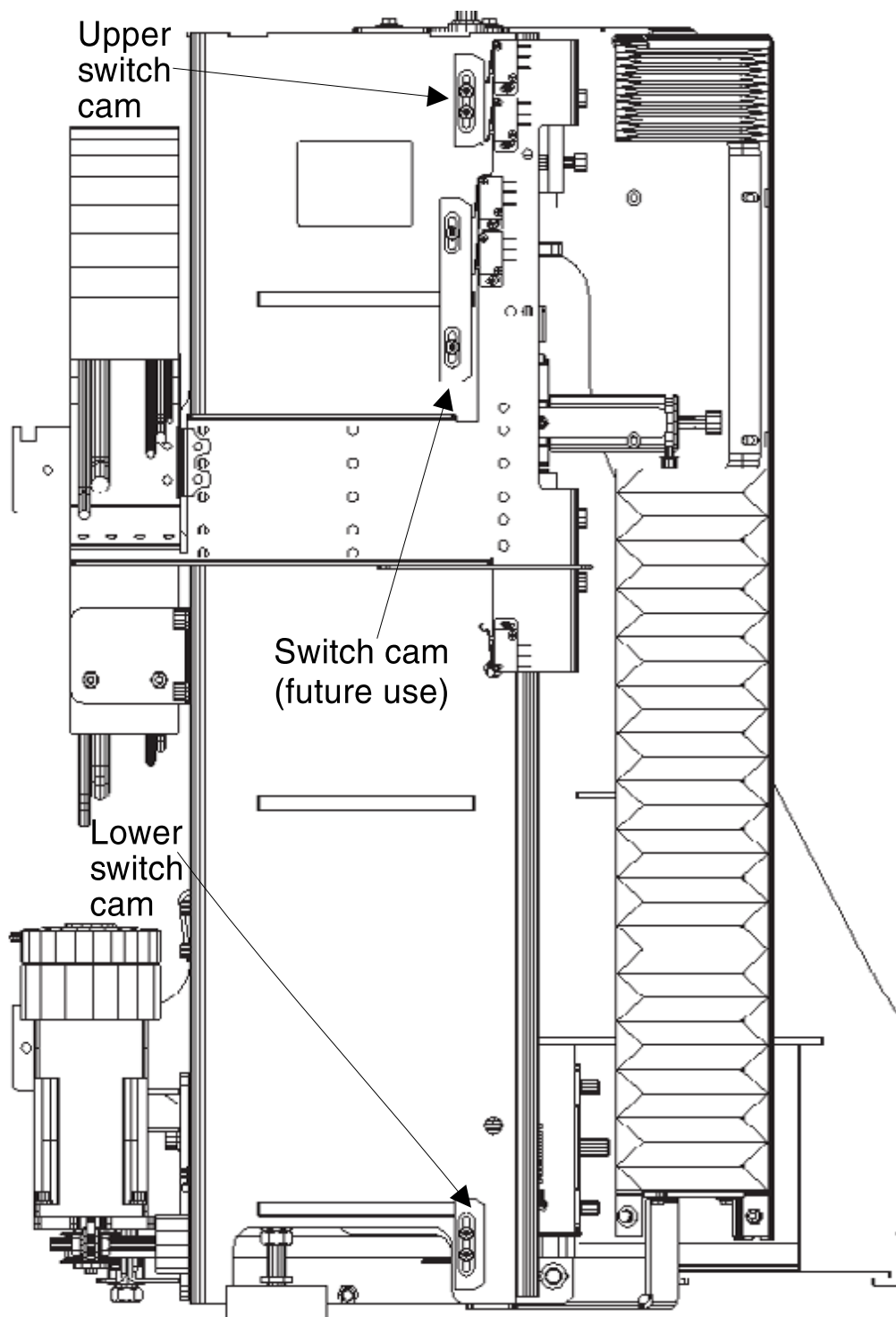
Fig. 25: Switch cams on lifting column
