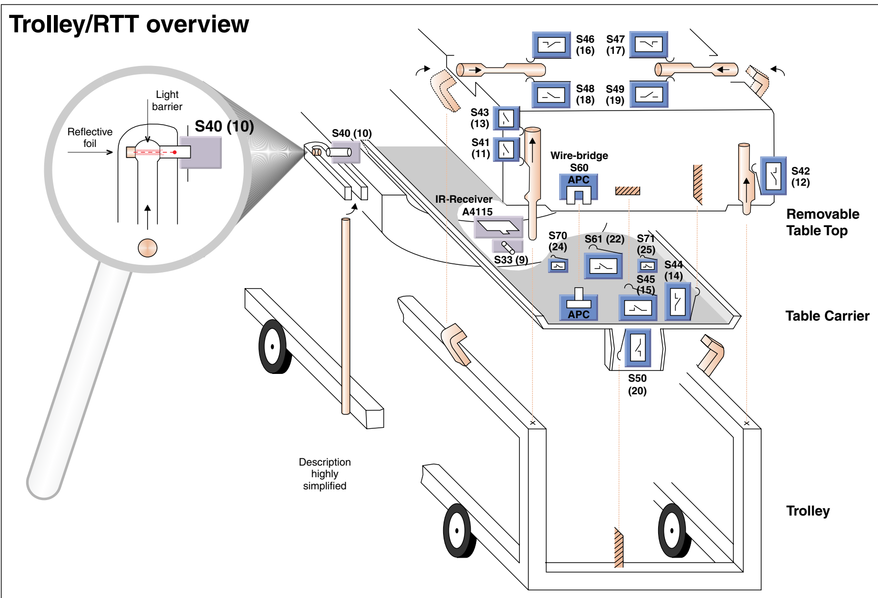
Fig. 31: Trolley/RTT Overview
