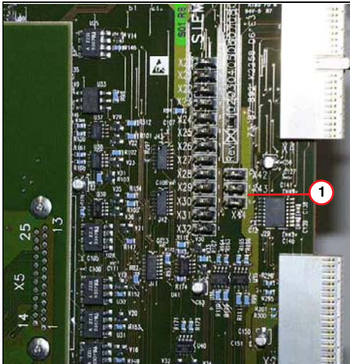
Fig. 9: Jumper setting D6 AMC Pos. 1 Jumper setting on D6 AMC X42-X44 1-2
