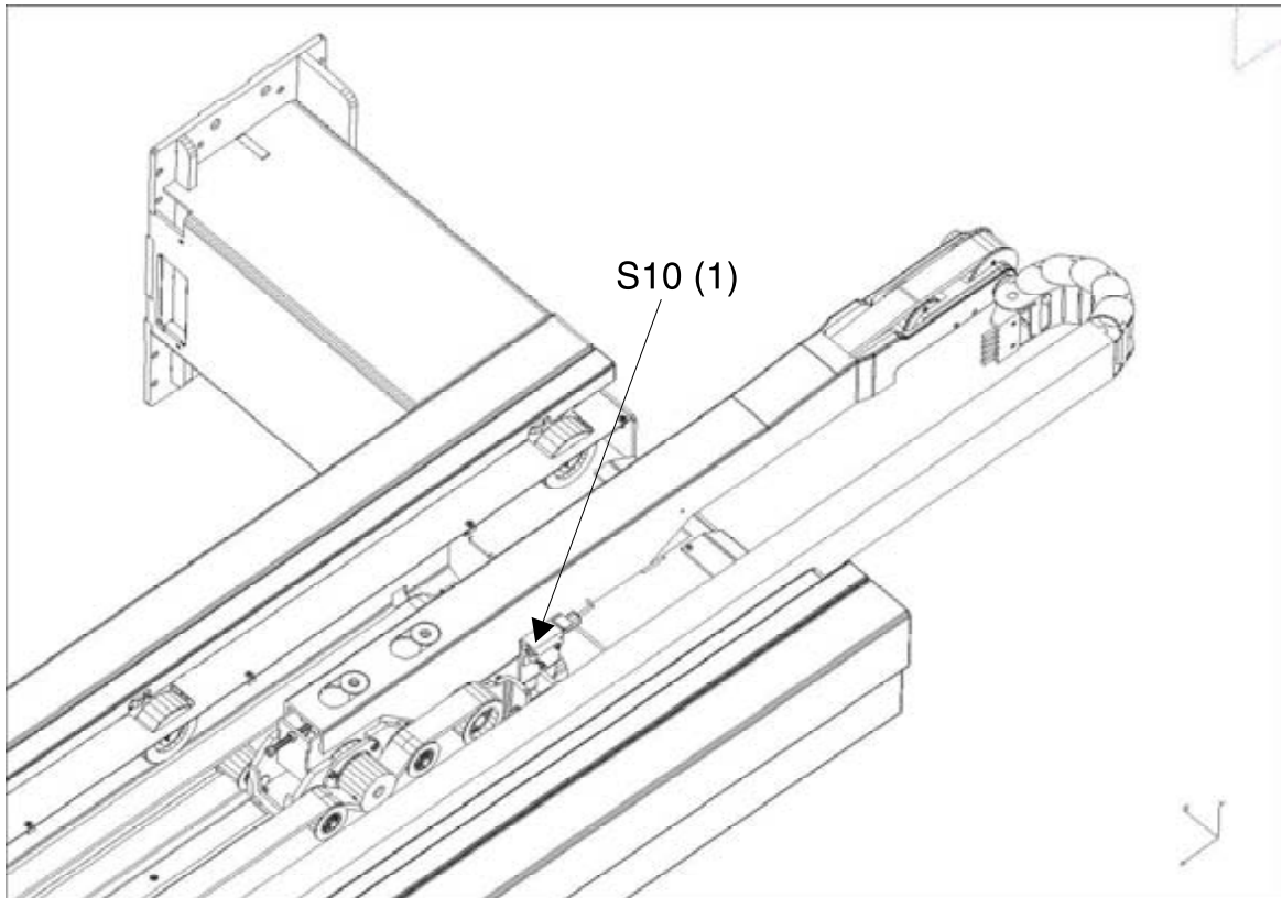
Fig. 30: Reference switch S10
